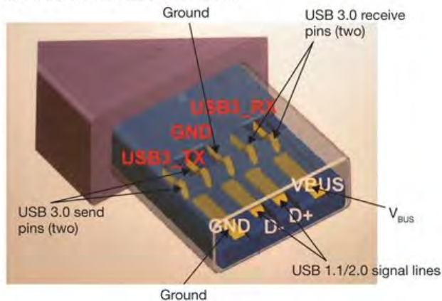
b) Pin layout for USB 3.0 connector
